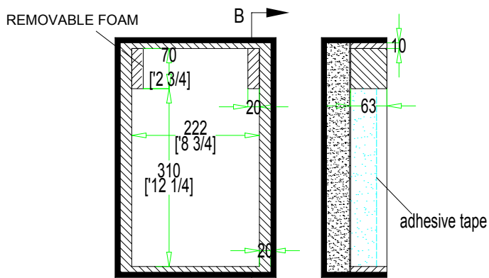
B-B VIEW
