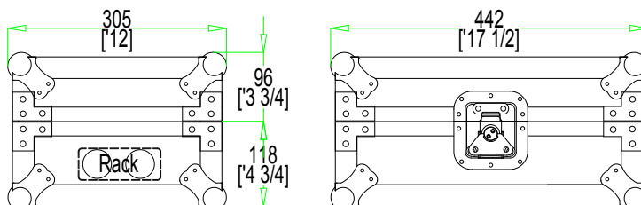
LEFT VIEW
