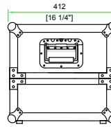
RIGHT VIEW
