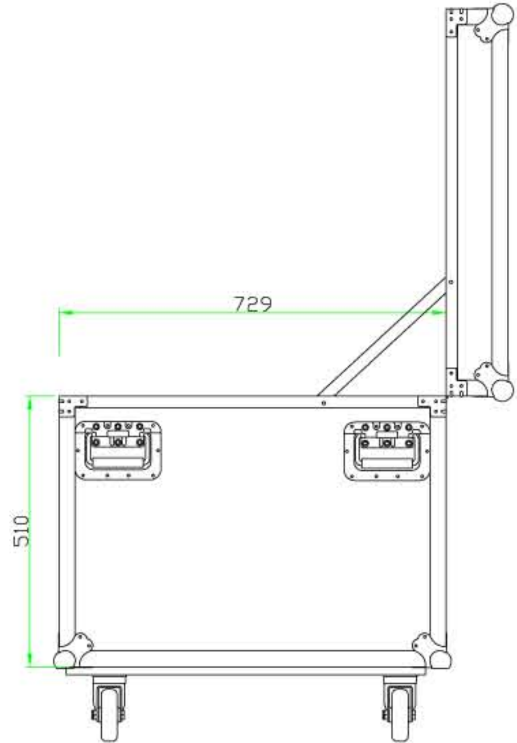
LEFT VIEW
