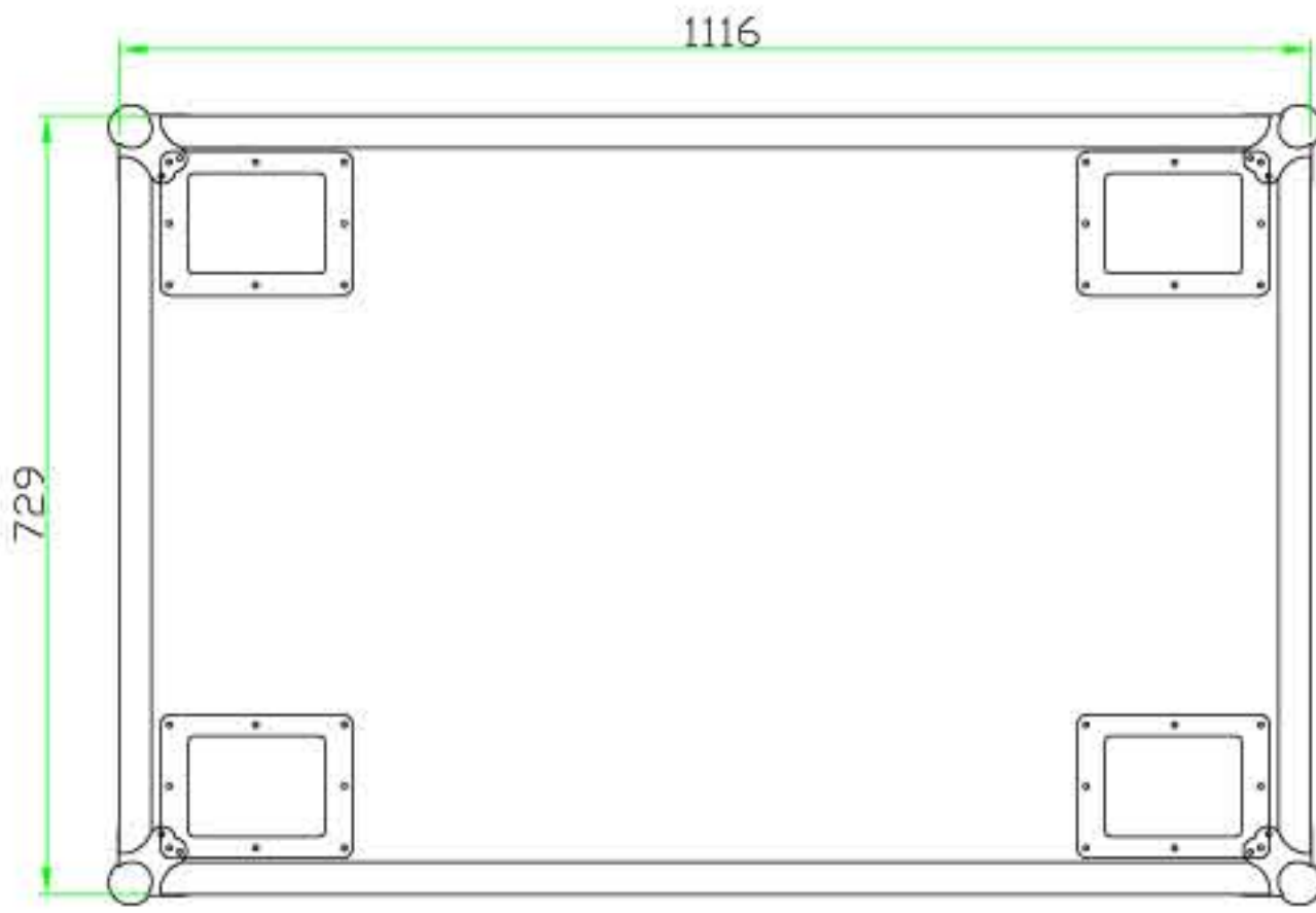
TOP VIEW
