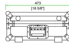
LEFT VIEW
