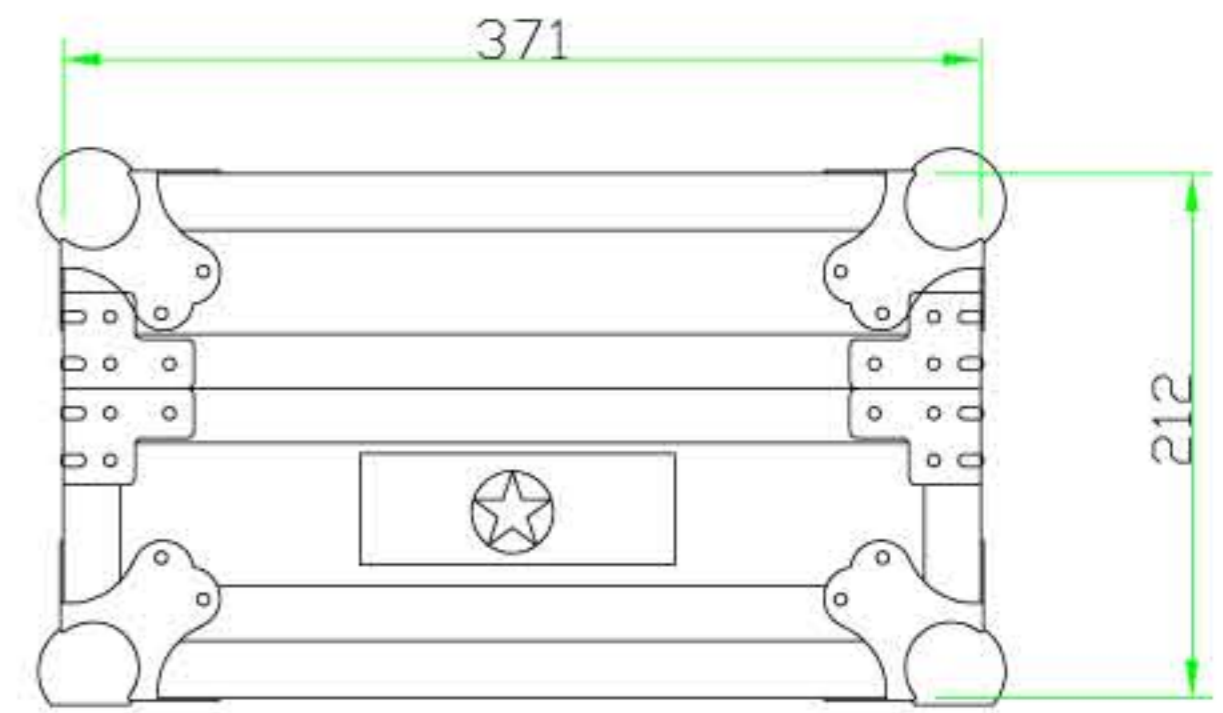
RIGHT VIEW
