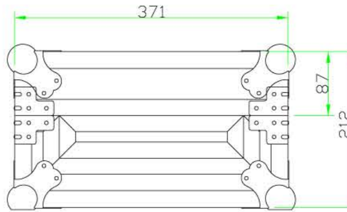
LEFT VIEW
