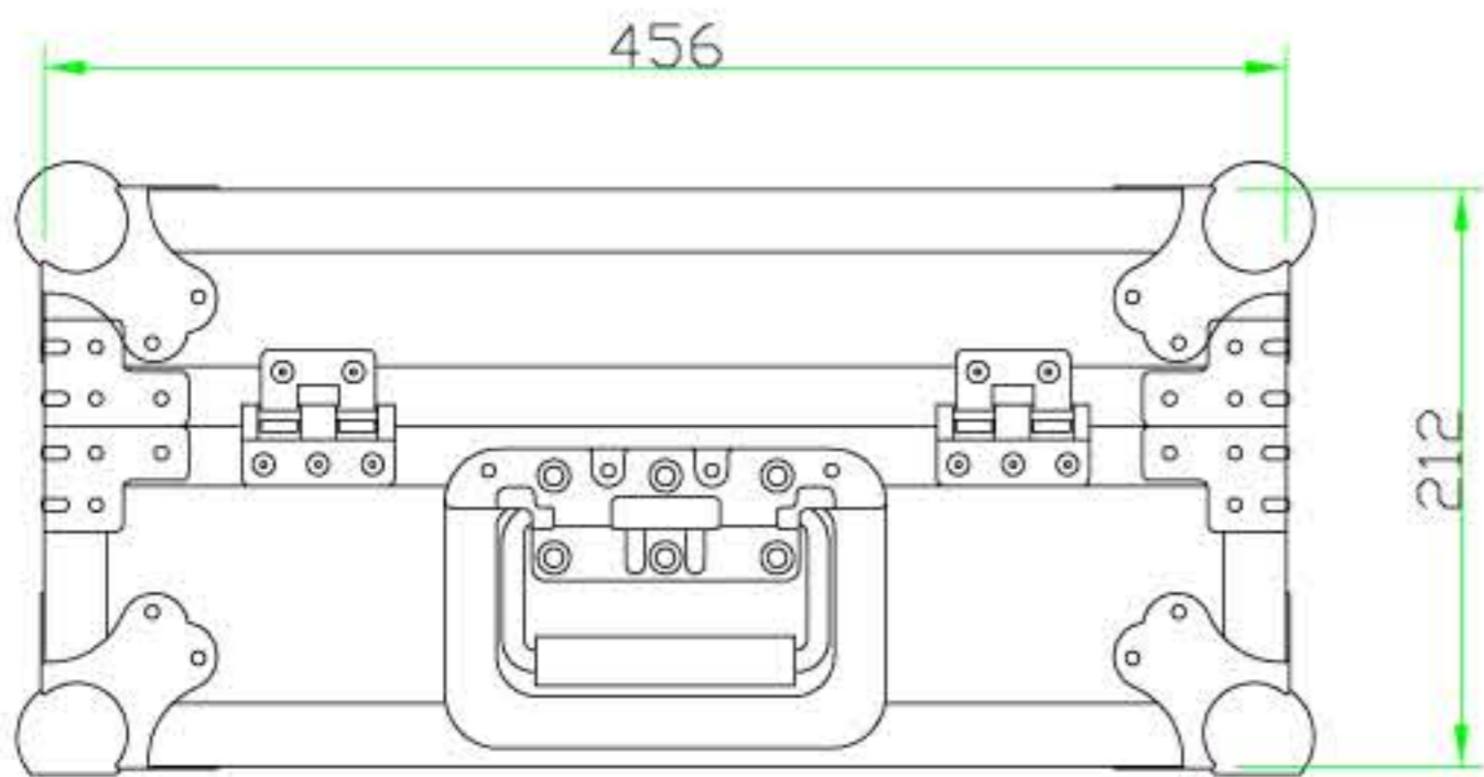
BACK VIEW
