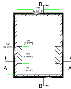
TOP VIEW OF COVER
