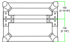
BACK VIEW
