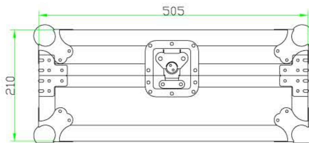
LEFT VIEW
