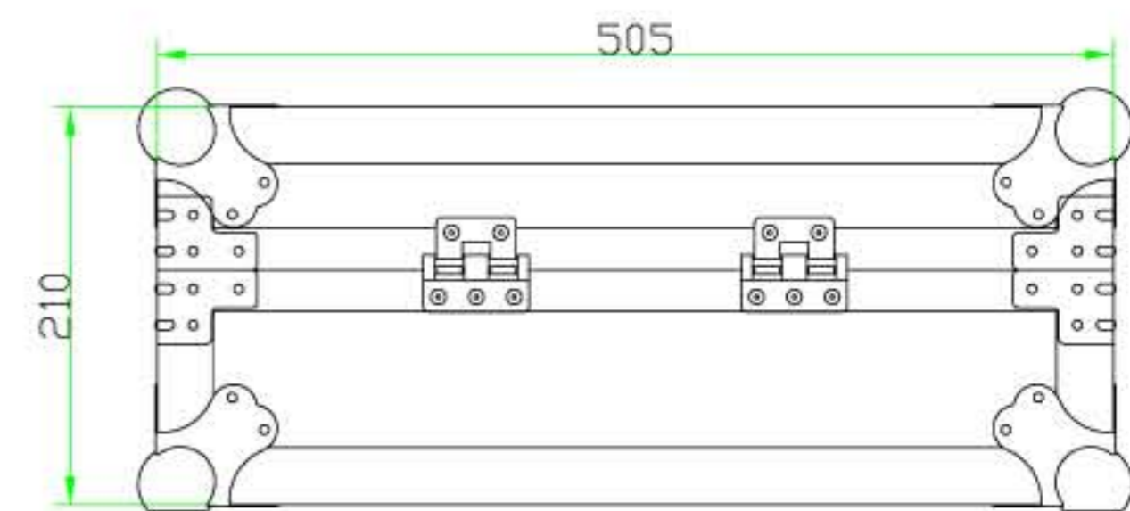
RIGHT VIEW
