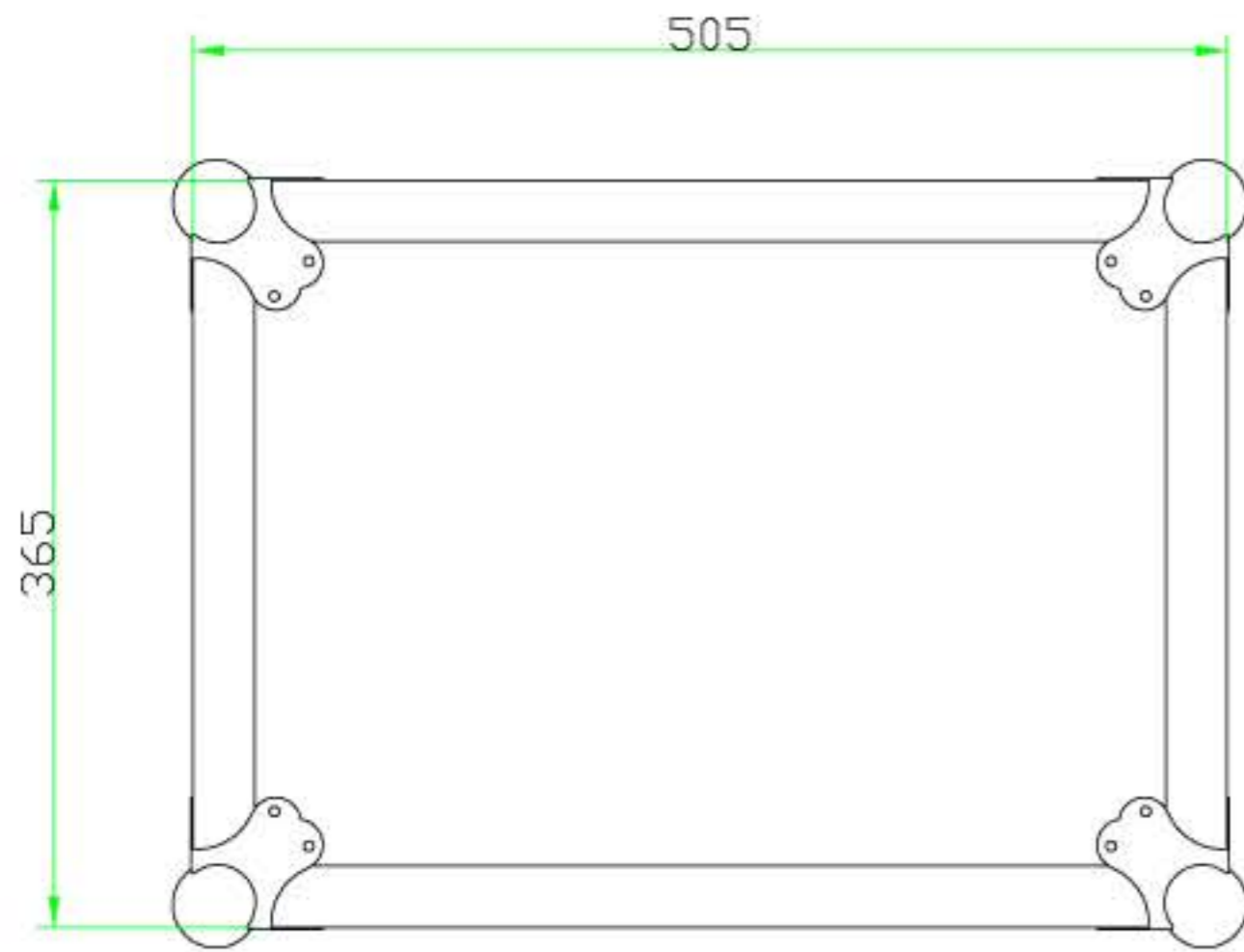
TOP VIEW
