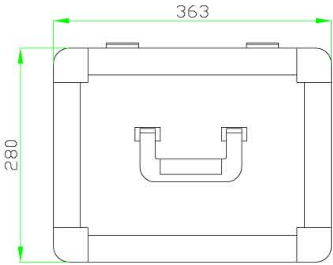
TOP VIEW
