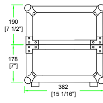
LEFT VIEW
