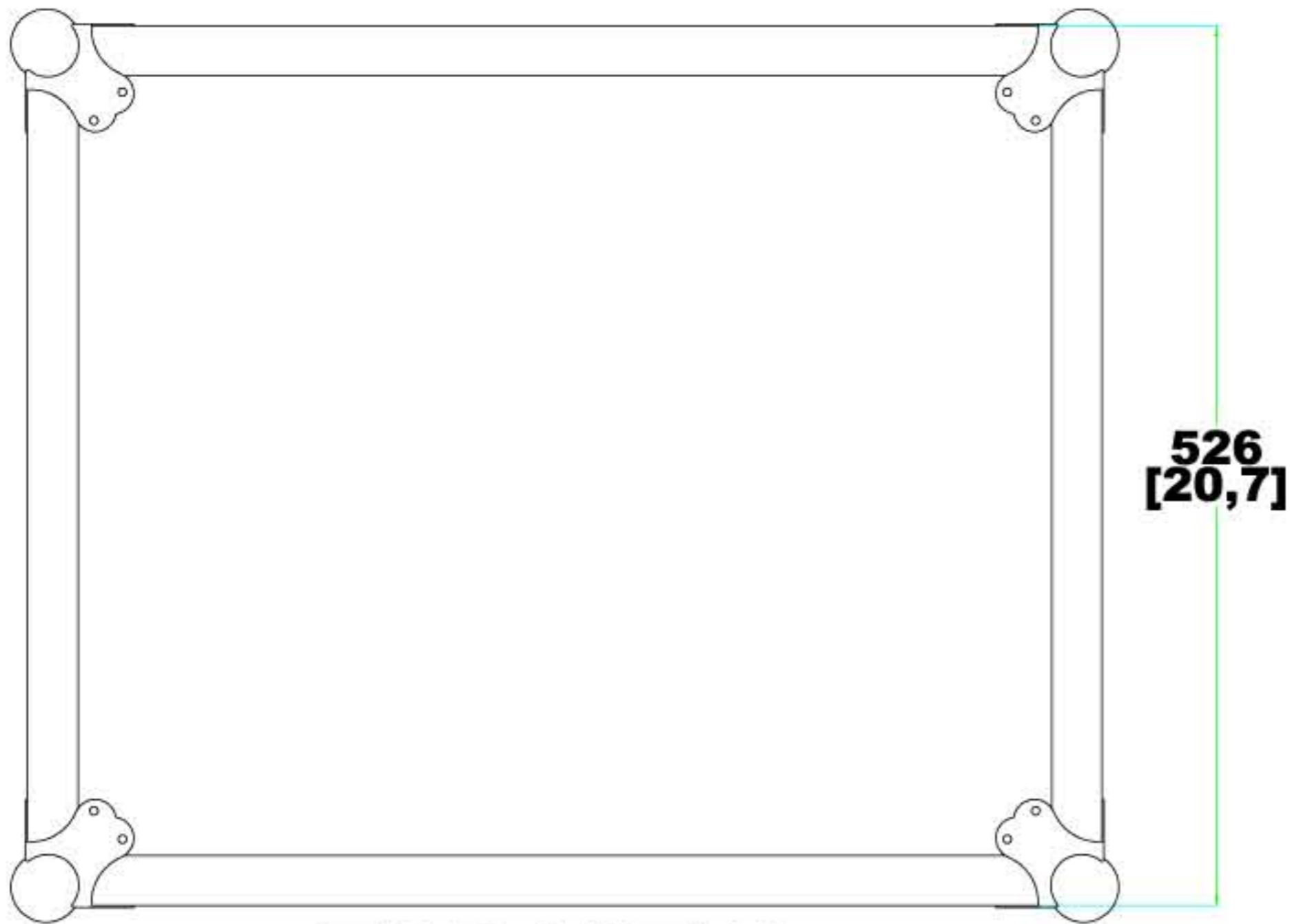
TOP VIEW
