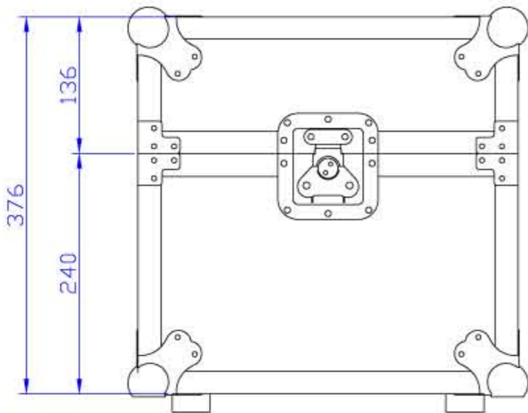
FRONT VIEW
