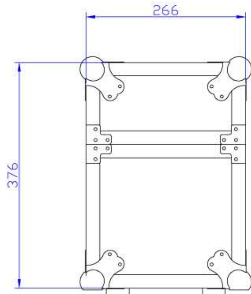
RIGHT VIEW
