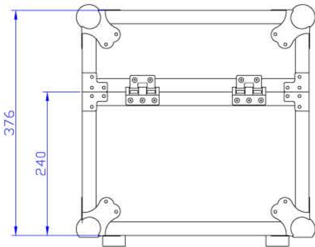
BACK VIEW
