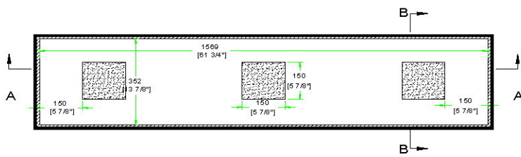
TOP VIEW OF COVER
