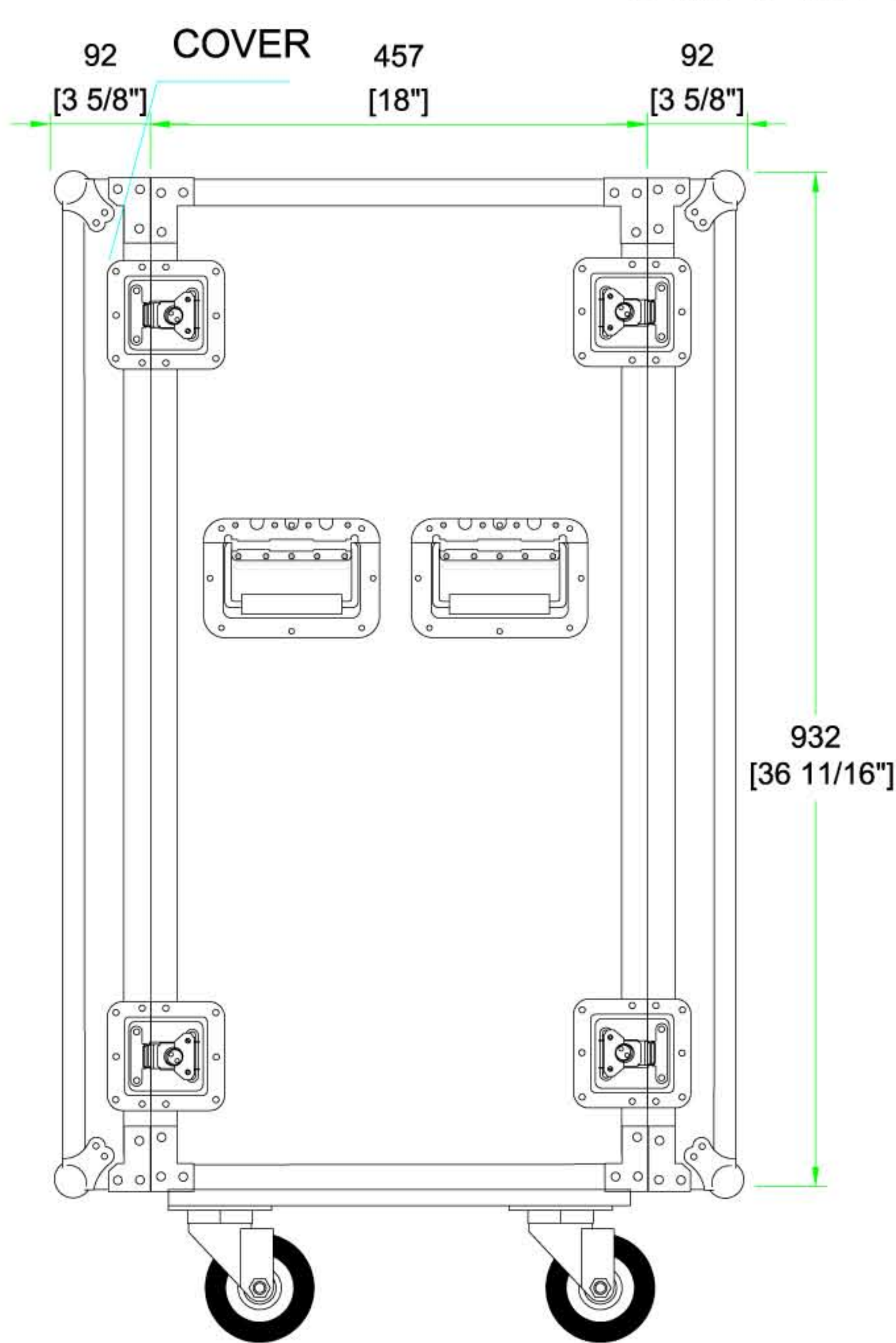
SIDE VIEW
