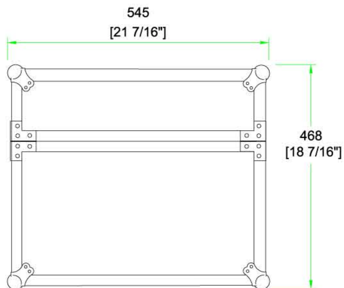
FRONT VIEW
