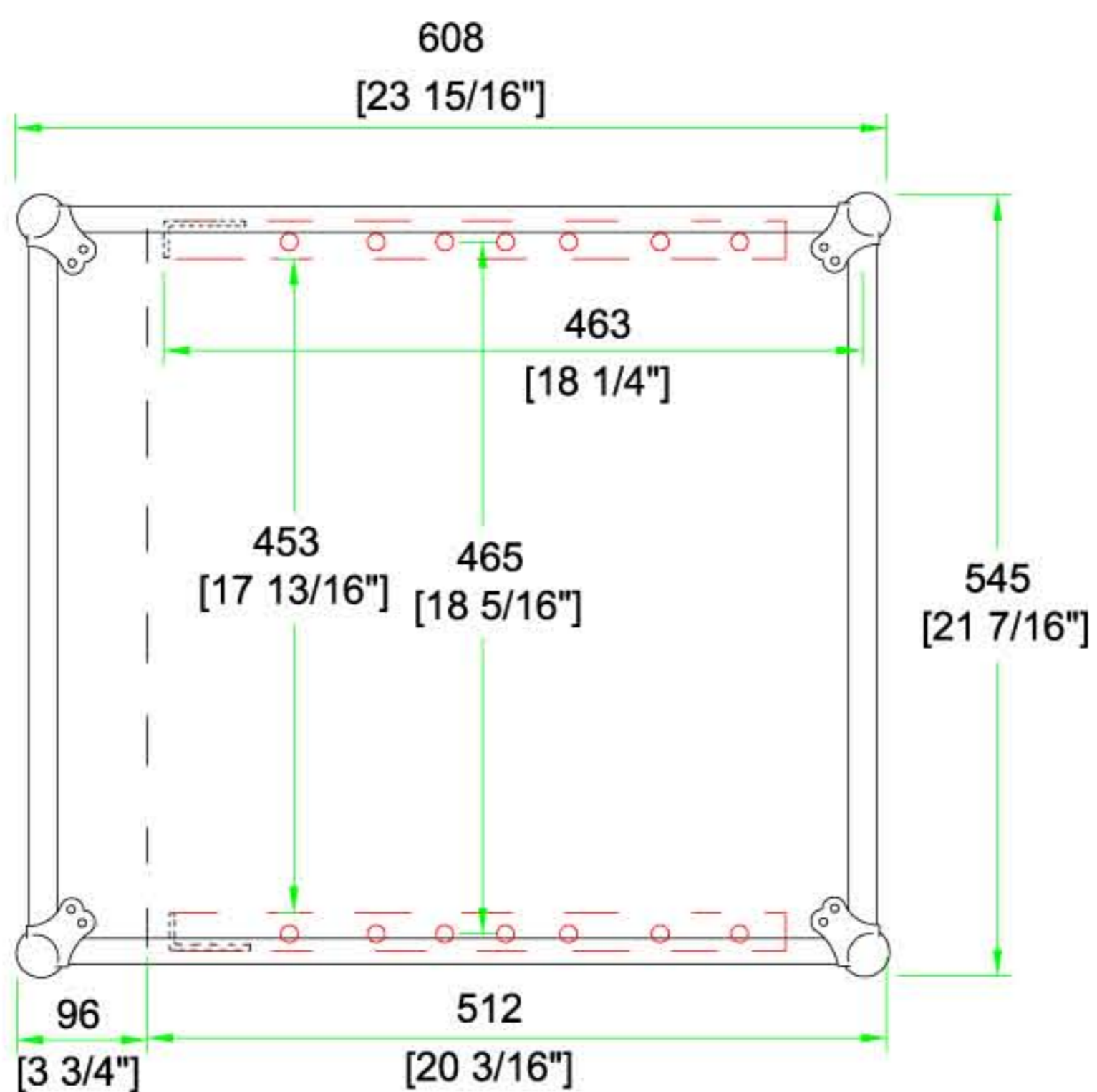
TOP VIEW
