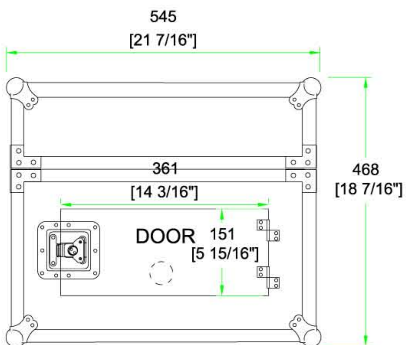
BACK VIEW
