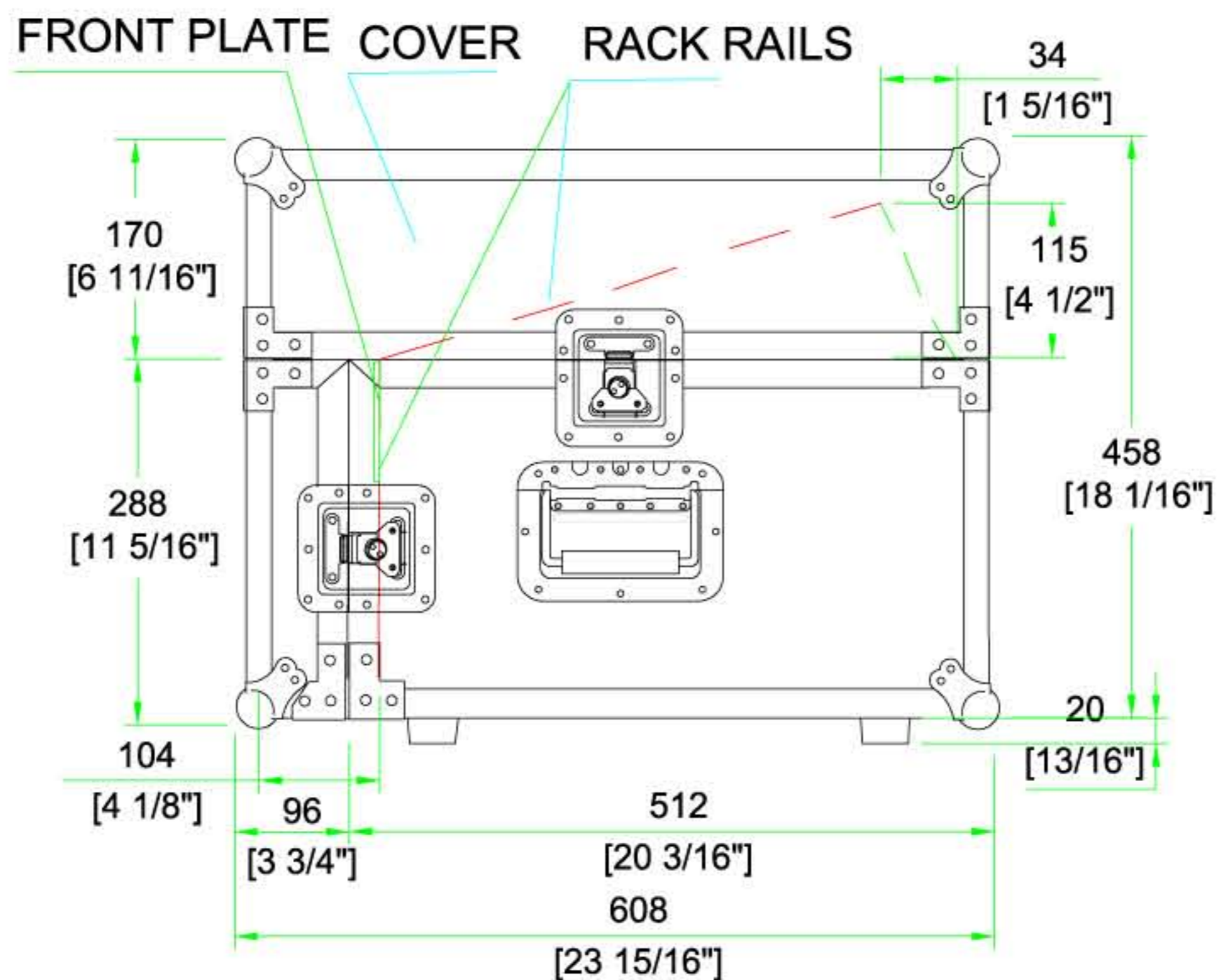
SIDE VIEW
