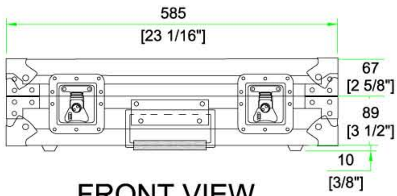
FRONT VIEW
