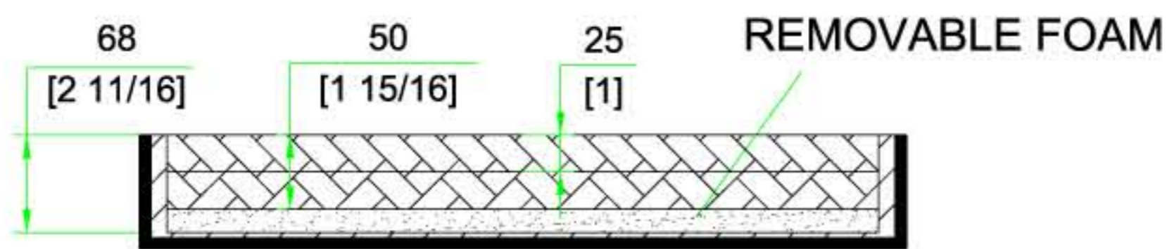
C-C VIEW
