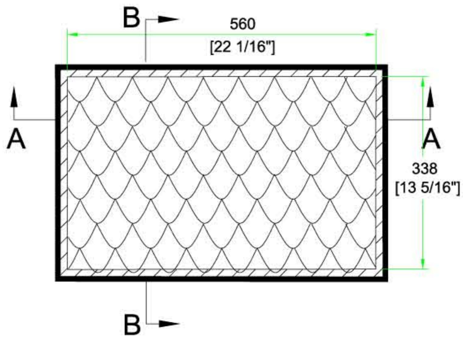
TOP VIEW OF COVER
