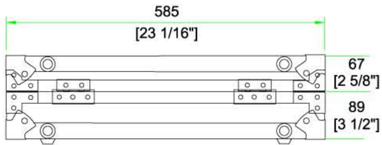
BACK VIEW
