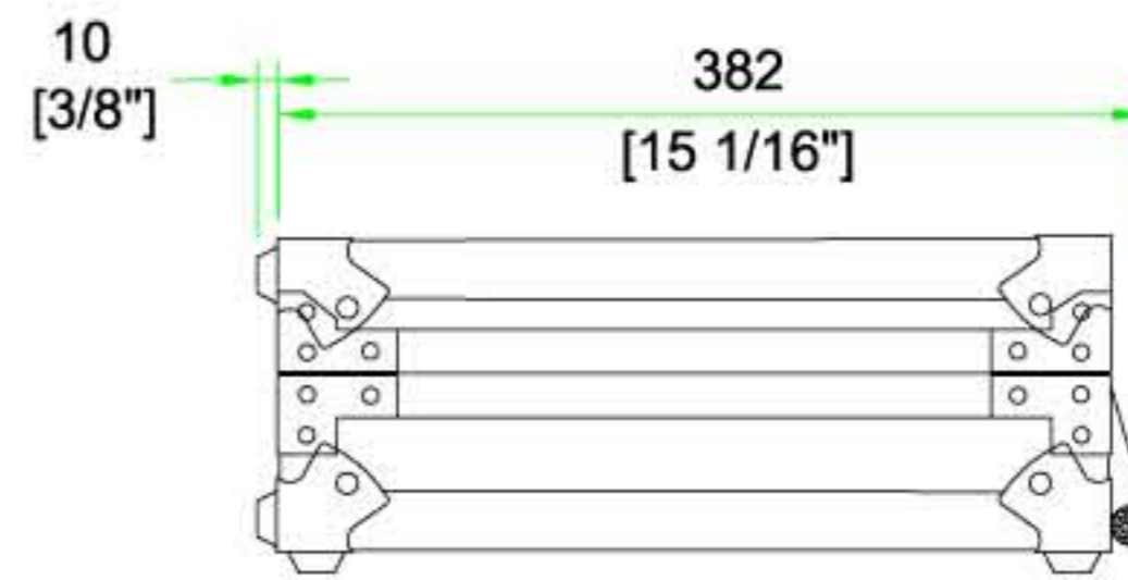
LEFT VIEW
