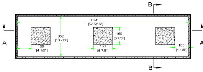
TOP VIEW OF COVER
