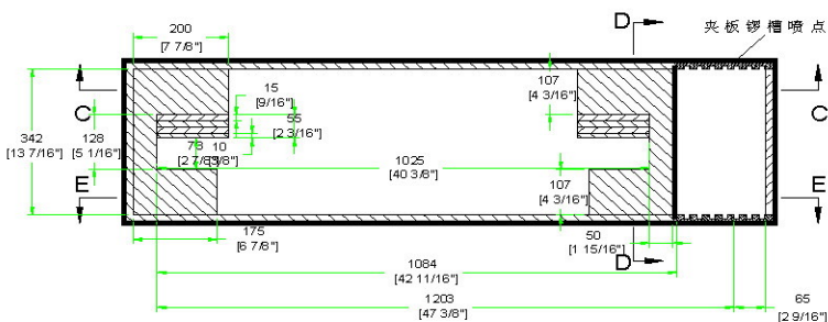
TOP VIEW OF BASE
