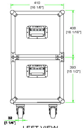
LEFT VIEW RIGHT VIEW
